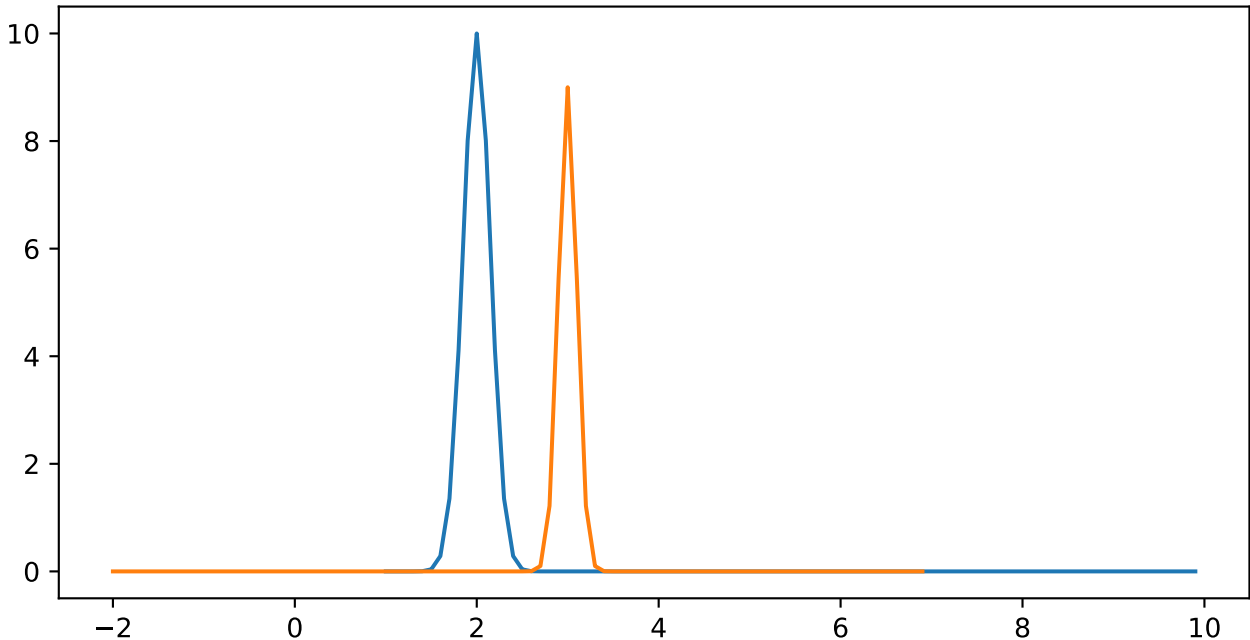
Evaluate two Gaussian1D models with 2 sets of input data
