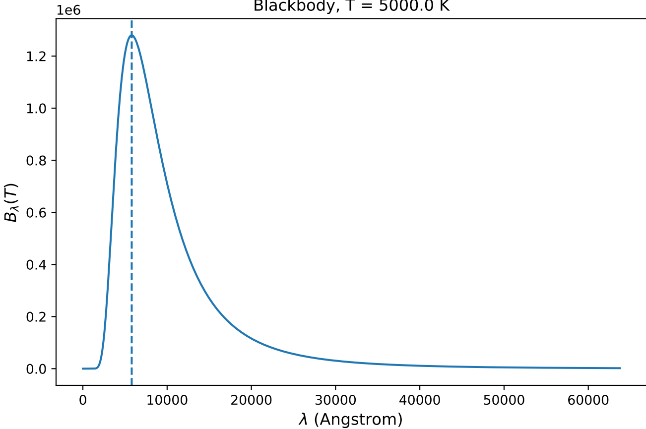
Blackbody, T = 5000.0 K
