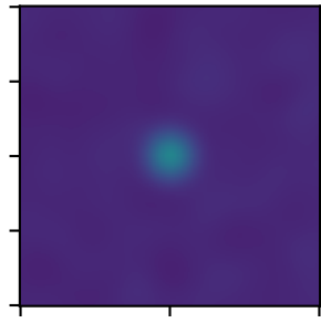
Gaussian2DKernel
