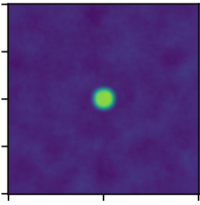
Tophat2DKernel
