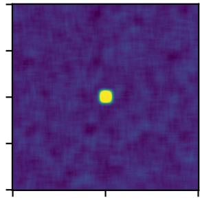
Box2DKernel
