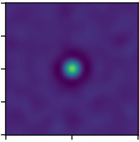
MexicanHat2DKernel
