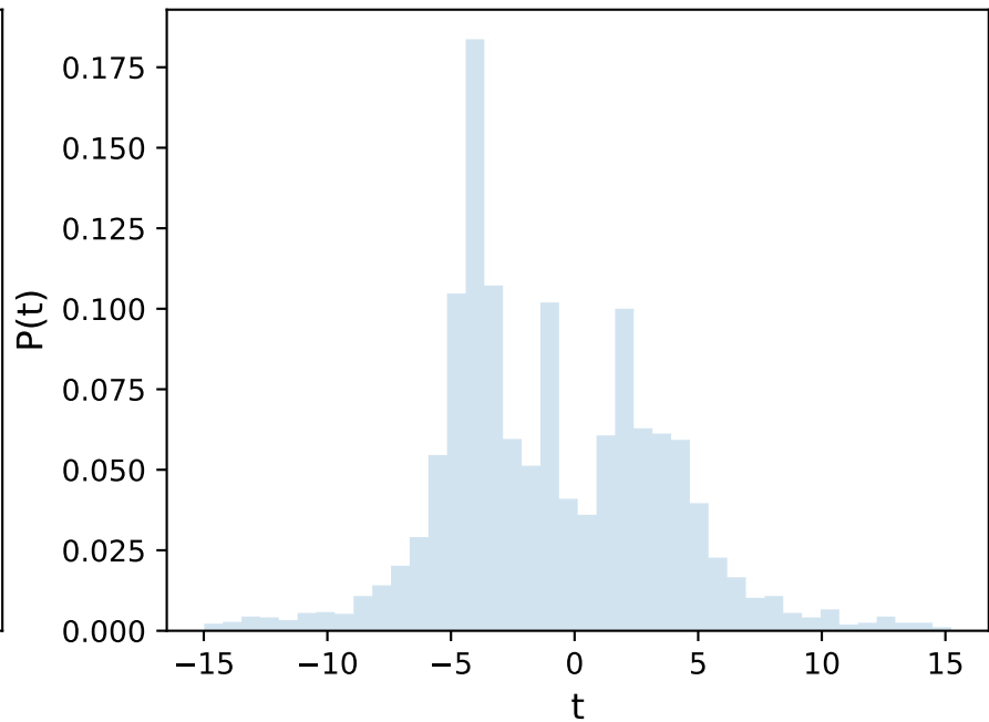
hist(t, bins="freedman")
