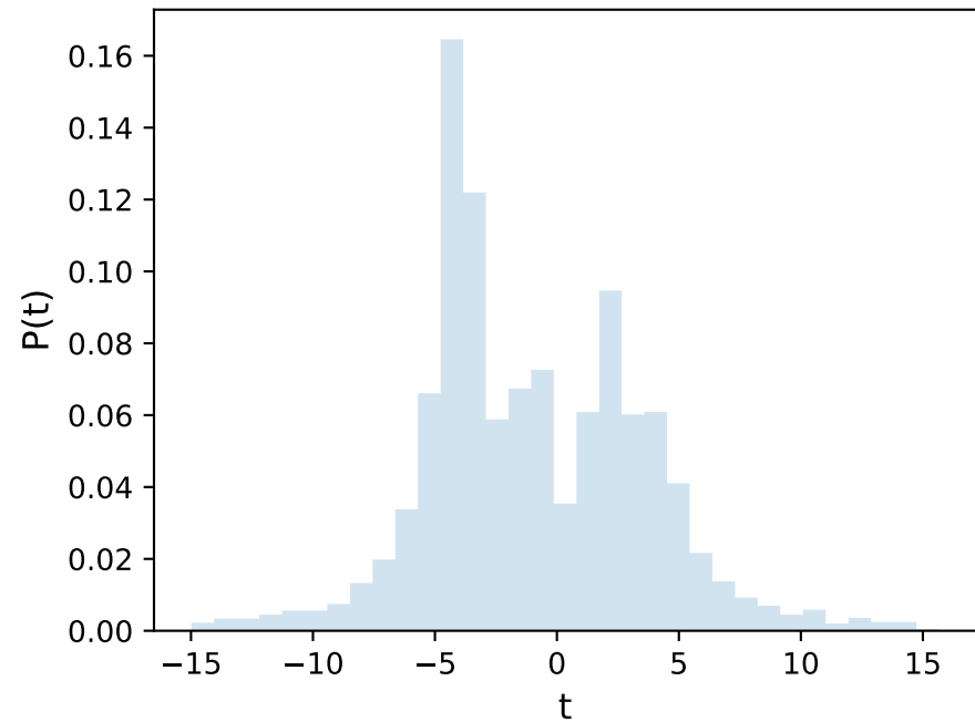
hist(t, bins="scott")
