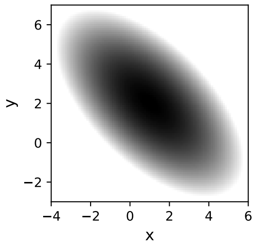
Sersic2D
