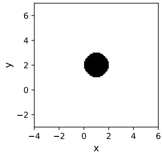
Moffat2D
