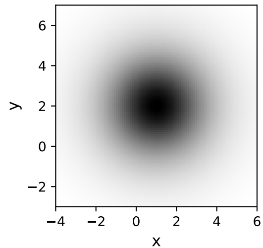
TrapezoidDisk2D
