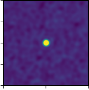
AiryDisk2DKernel
