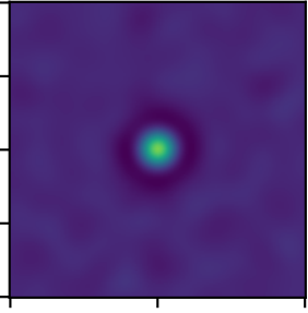
RickerWavelet2DKernel
