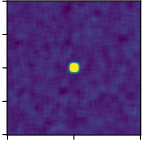
Box2DKernel
